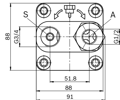
View X
